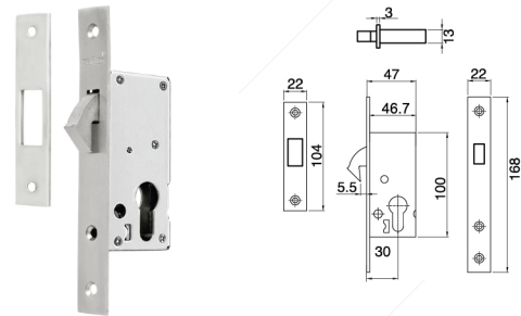
MTS SLD DL 83100 SSS
