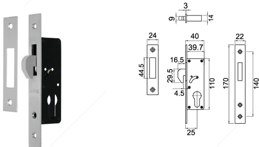
MTS SLD DL 8225 SSS
