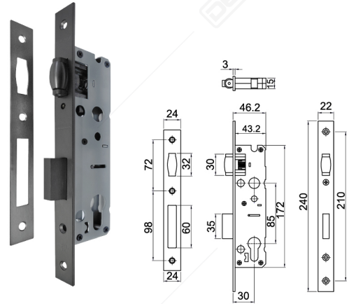
MTS RL DL84030 GUN METAL
